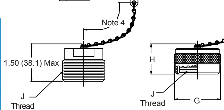
TYPE A - Plug Cap For use with MS17344
