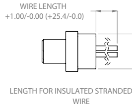
Wire Harness Side View
