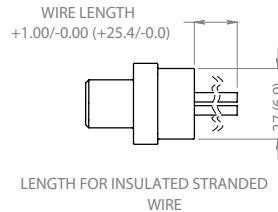
Wire Harness Side View
