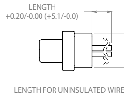
Wire Harness Side View
