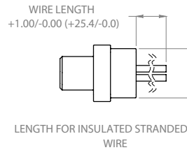
M22759/11-26 Type Teflon-Insulated Hookup Wire - 36 Inches (914mm), White Front View
