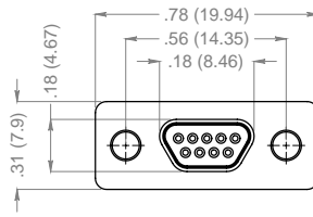
Wire Harness End View
