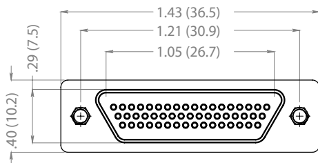
PCB Mounted Compact Straight End View
