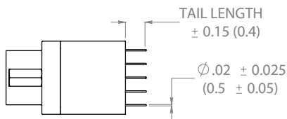
PCB Mounted Compact Straight Side View
