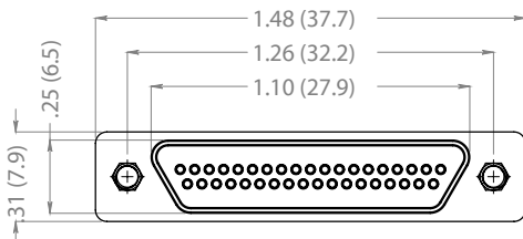
PCB Mounted Compact Straight End View
