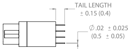
PCB Mounted Compact Straight Side View
