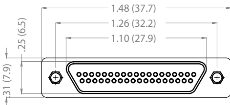
PCB Mounted Compact Straight End View
