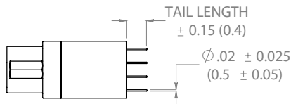
PCB Mounted Compact Straight Side View
