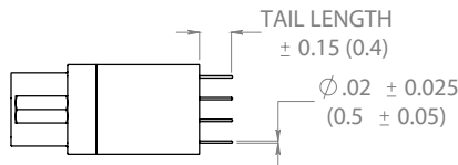
PCB Mounted Compact Straight Side View
