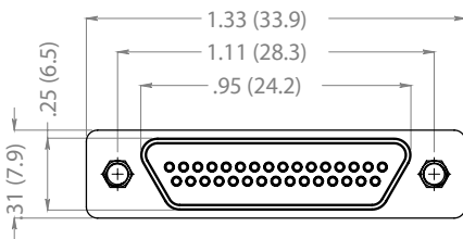
PCB Mounted Compact Straight End View
